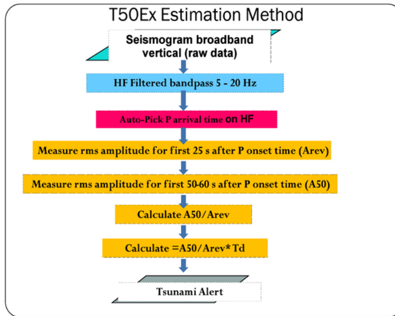
Figure 4. Direct procedure to estimate P-wave T50Ex
