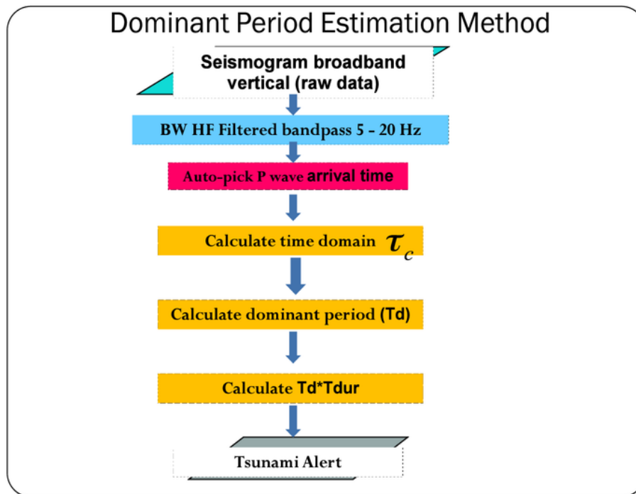
Figure 3. Direct procedure to estimate P-wave dominant periods
